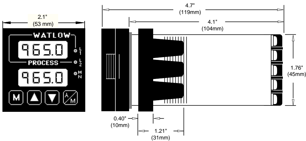
Figure 3 - Series 965 Dimensions
