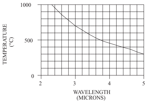
Quartz Infrared Radiant Heater Emission Wavelength vs Temperature 300° - 850°C (Useful Range)
